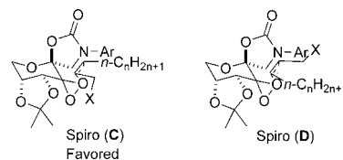
Figure 3. Stereodifferentiation via hydrophobicity.
