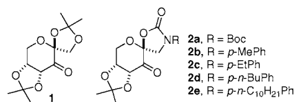
Figure 1. Ketones 1 and 2 .
