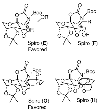
Figure 4. Transition states for ether/ketal-containing olefins.
