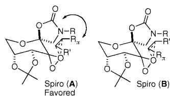
Figure 2. Transition states for the epoxidation with ketone 2 .
