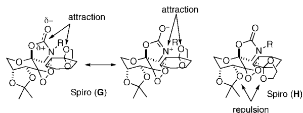
Figure 5. Possible electronic interactions in transition states.
